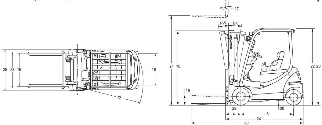
Dimensions/AE50 Series
