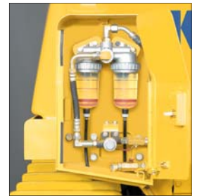
Large water separator
